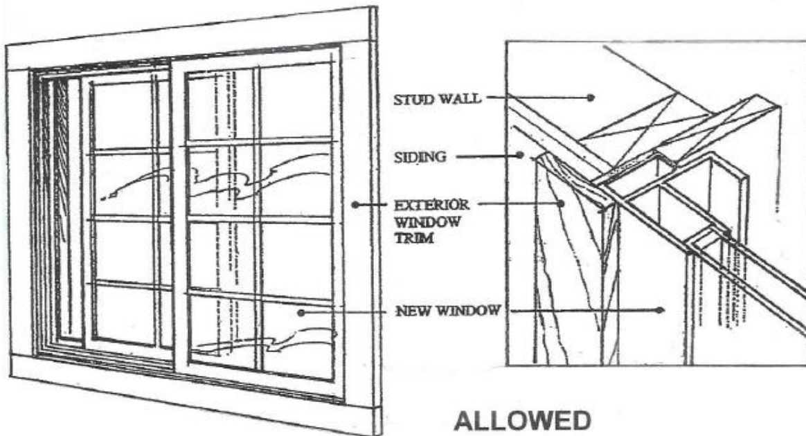
Acceptable Installation
