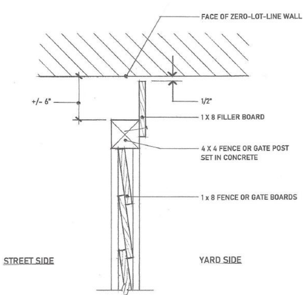
FENCE-TO-WALL DETAIL (Zero-Lot-Line Walls)
