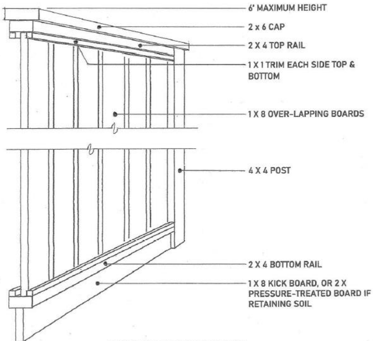
STANDARD FENCE DETAIL
