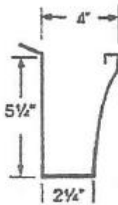
FASCIA GUTTER WITH CURVED FACE
