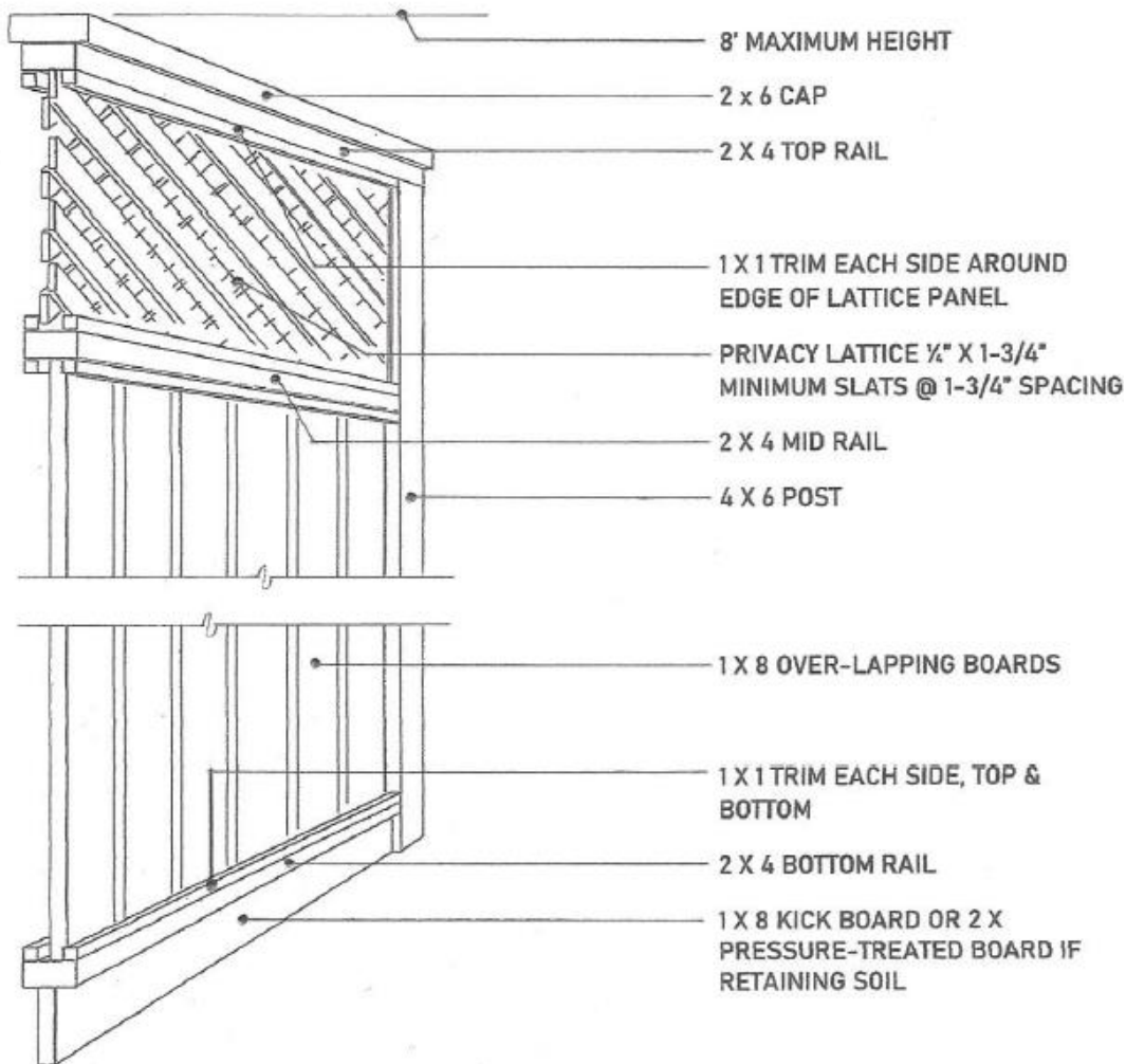
STANDARD FENCE EXTENSION DETAIL
