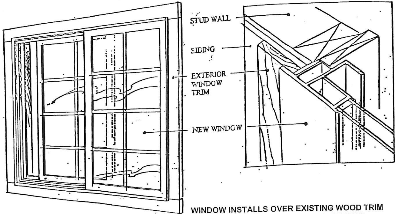
UNACCEPTABLE INSTALLATION
