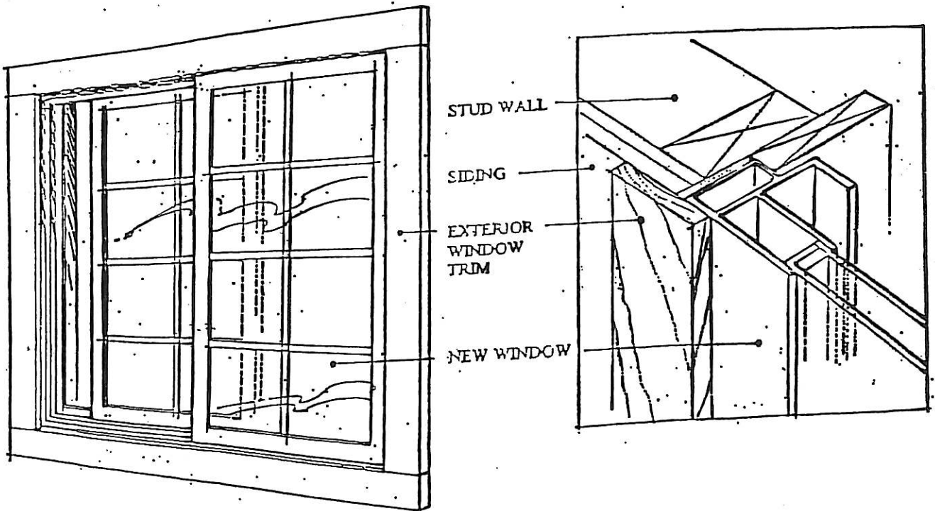
ACCEPTABLE INSTALLATION
