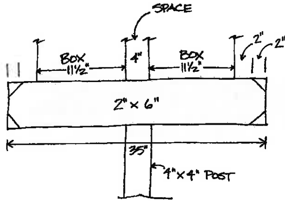
Double Box Configuration
