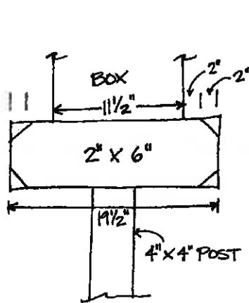
Single Box Configuration
