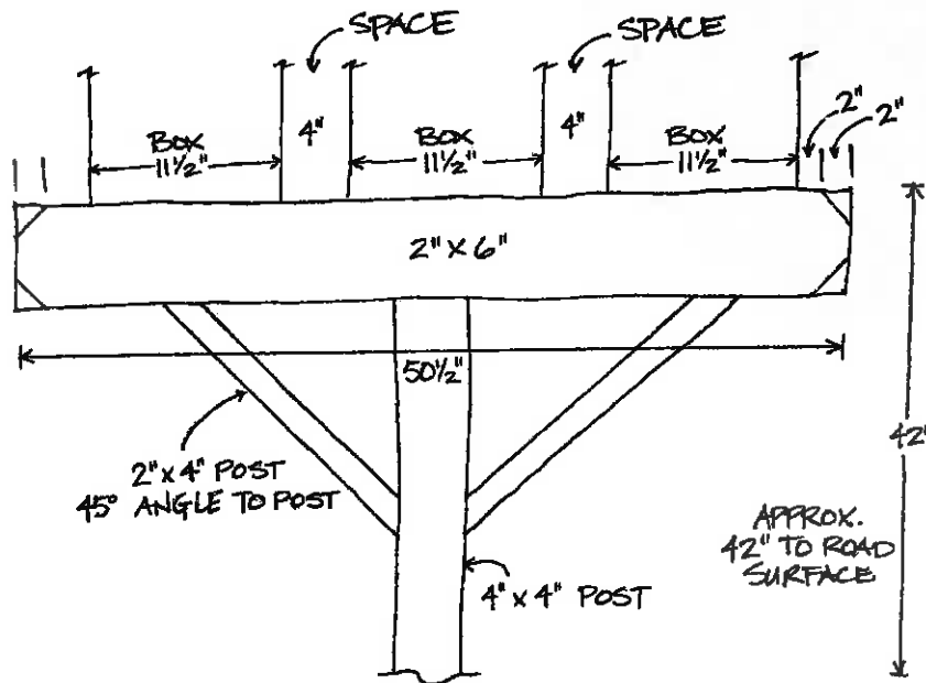
Triple Box Configuration
